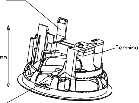
Locking ribs on each side. Secure loudspeaker to ceiling
